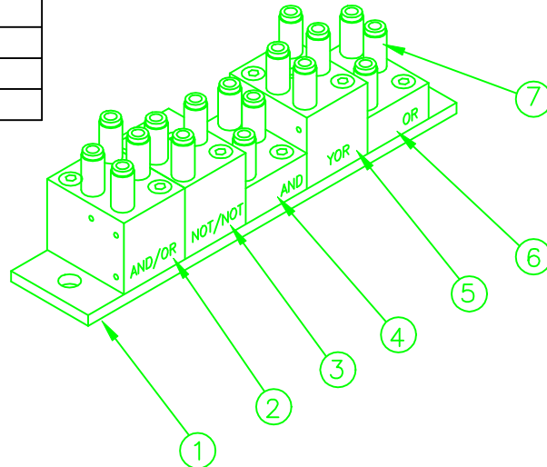
One-Hand Control Valve Pack (Part No. A-3321)
